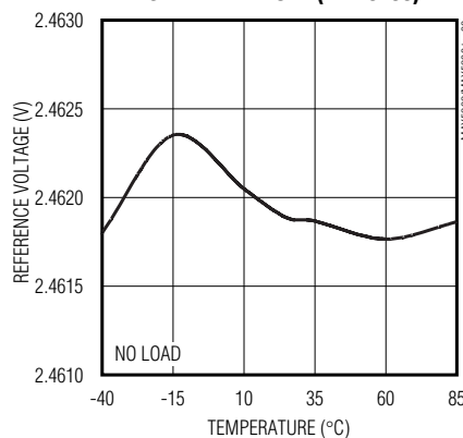
REFERENCE VOLTAGE vs. TEMPERATURE (MAX5233)
